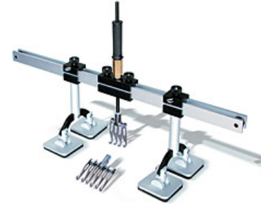
1) Dent lifter L 850 complete with feet, pulling handle, 2 claws.
